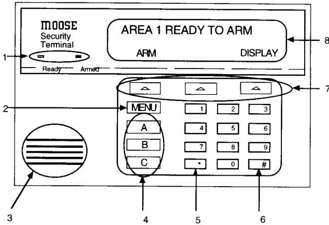
FIGURE 1 - LCD CONTROL STATION
