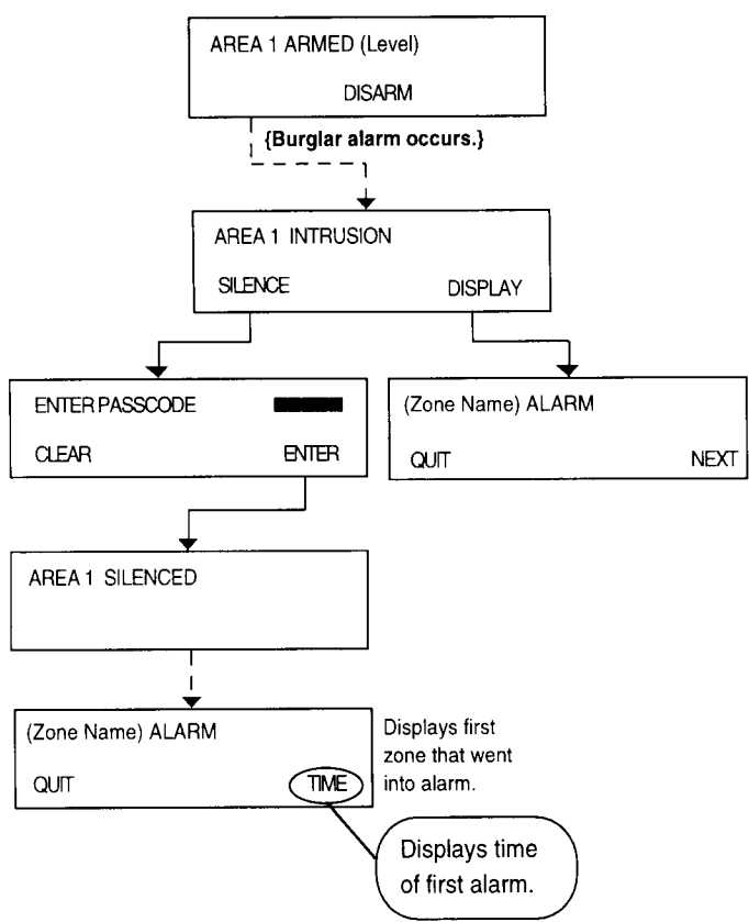
FIGURE 10 - SILENCING AN ALARM
